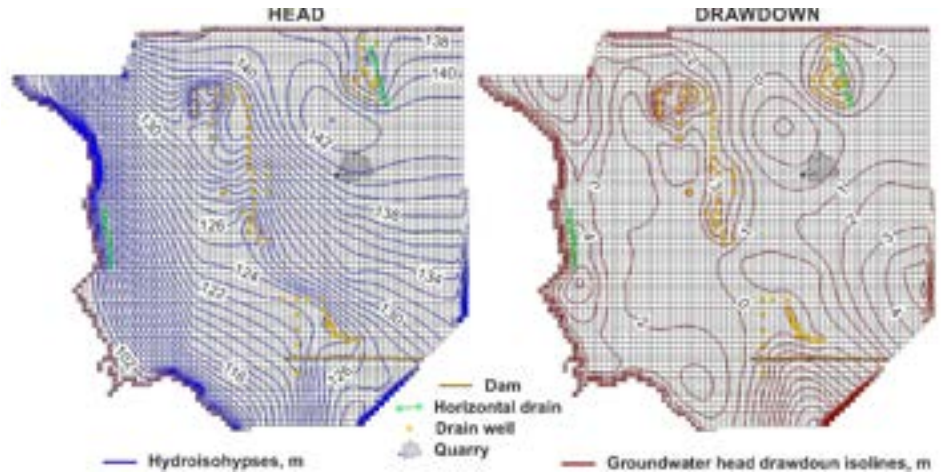
Fig. 6. Groundwater level and Drawdown map by 2030 year, developed based on prediction modelling results of the third scenario of drainage system work
